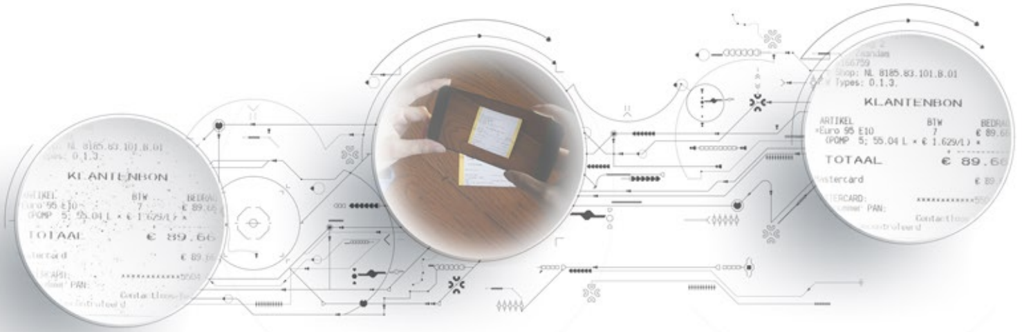
Normal Binarization
